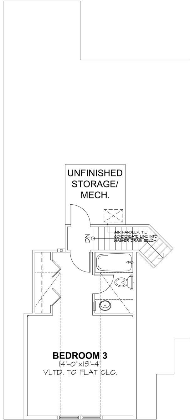
BONUS FLOOR PLAN
